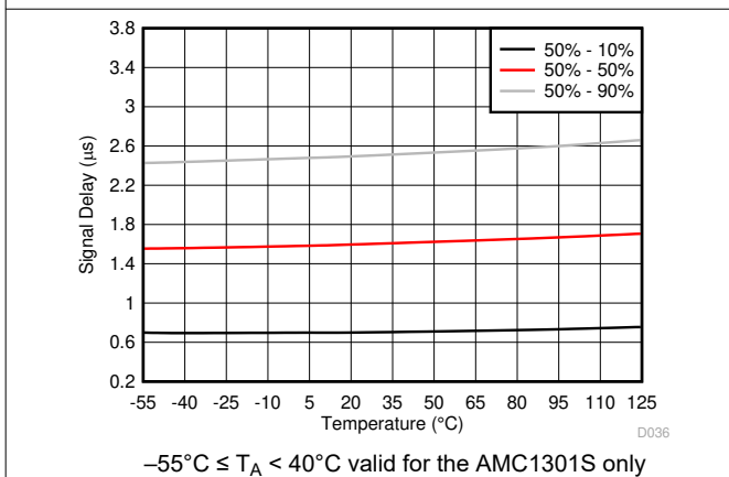
Figure 6-39. V IN to V OUT Signal Delay vs Temperature
