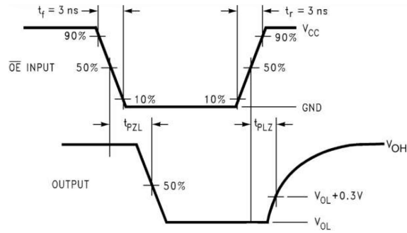
Figure 6. AC Waveforms
